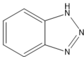
Figure 1. Benzotriazole nucleus
